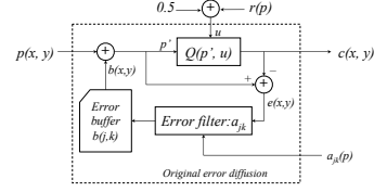
Figure 1: The principle of the standard error-diffusion.
