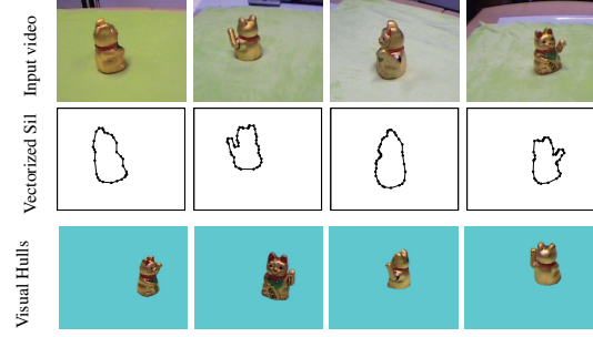
Figure 7: Silhouettes vectorization in eight video streams and Visual Hull rendering based on the silhouettes. The first row shows 4 channel video images(eight in total), the second row is the corresponding vectorized silhouettes. Visual hulls are rendered from different viewpoints based on the silhouettes(the third row).
