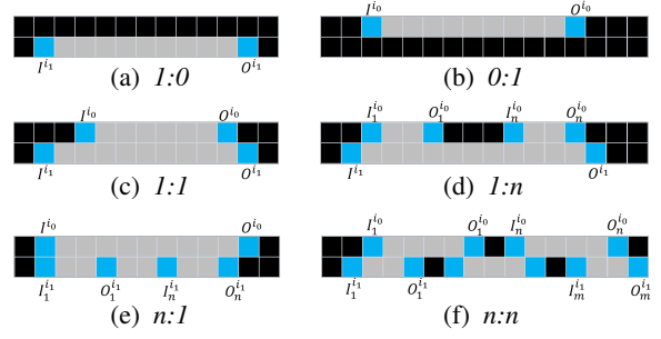
Figure 3: Six cases of the connectivity relationship between intervals on two adjacent lines.
