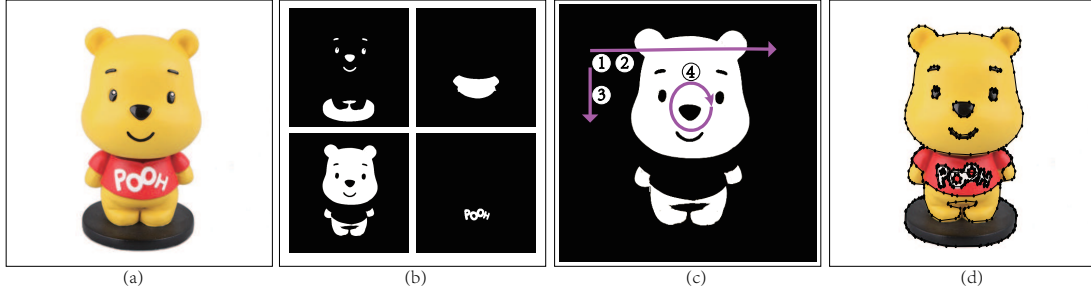
Figure 1: Vectorizing a cartoon color image with our method. (a)The input raster image. (b)The binary silhouettes. (c)The main procedure of our algorithm:①parallel boundary detection and ②precontouring, ③ sequential contouring and ④parallel contour vectorization. (d)The vectorization result. The contours are represented by line segments. The whole computation is completed in 9ms, which provides possibility for real-time applications.
